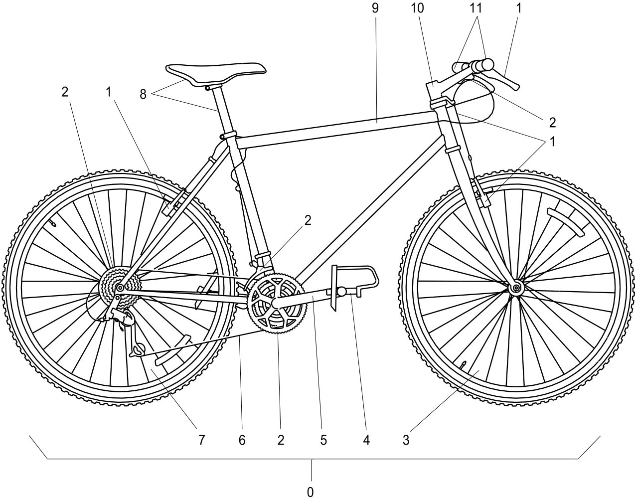
Fig 1 Complete bicycle
