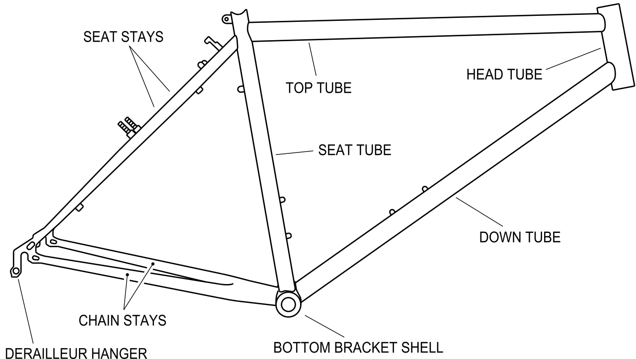
Fig 2 Frame
