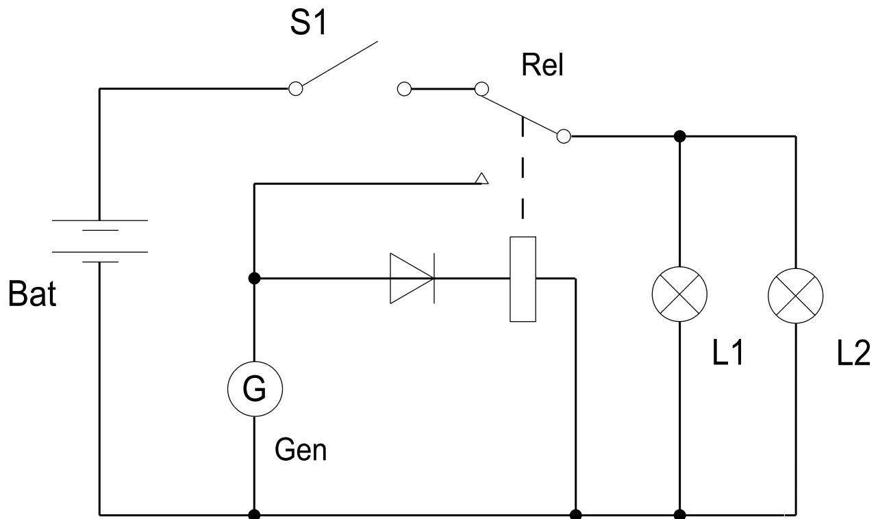
Fig 1 Lighting system
